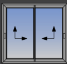
Double lifting sliding sash with narrow interlocking profile
